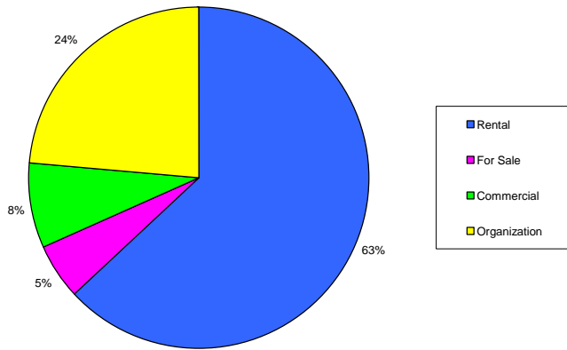
Loan Portfolio by Use 6-30-10
